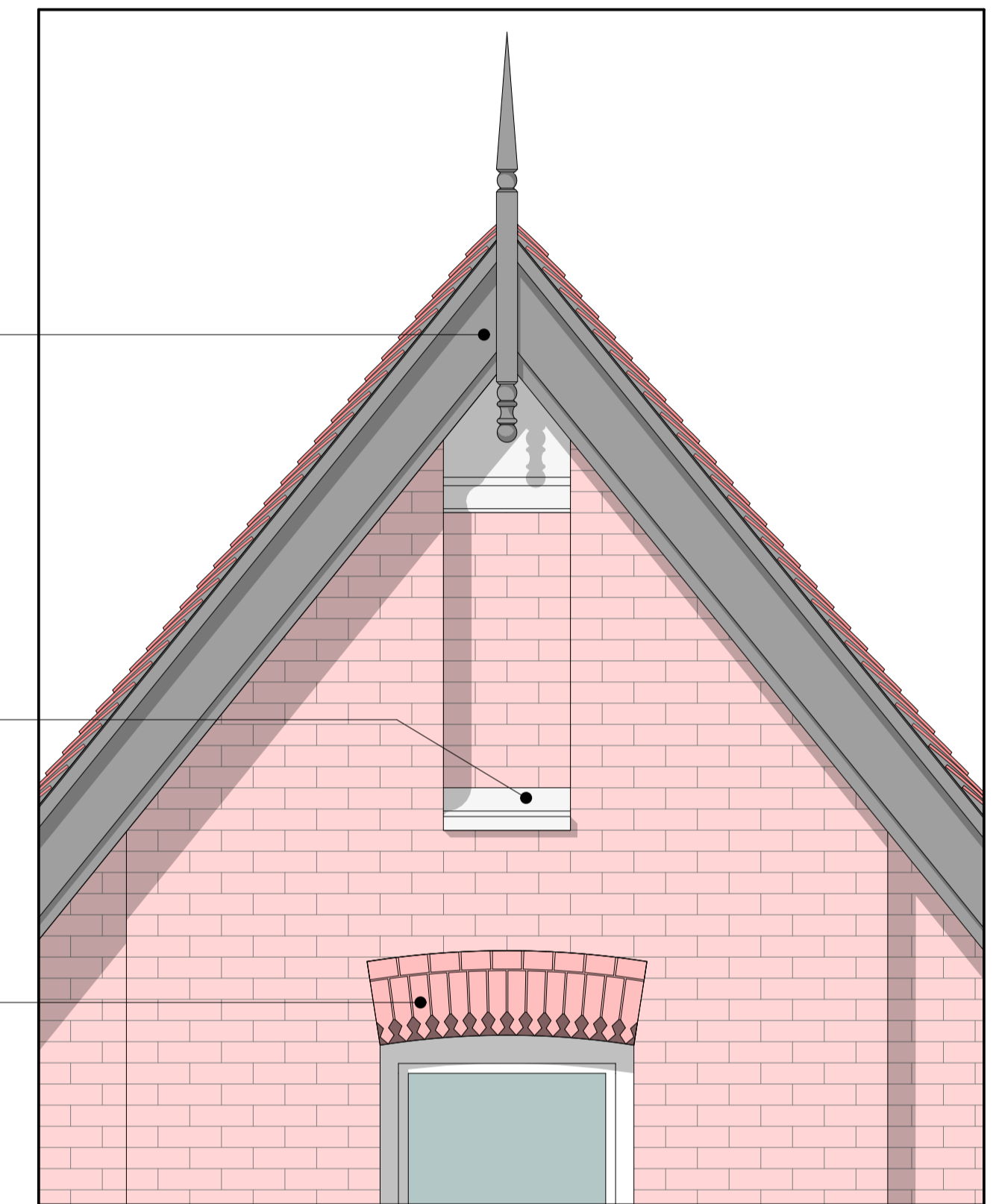
GABLE DETAIL
